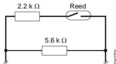
NAMUR circuitry
