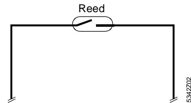
Reed contact without NAMUR circuitry
